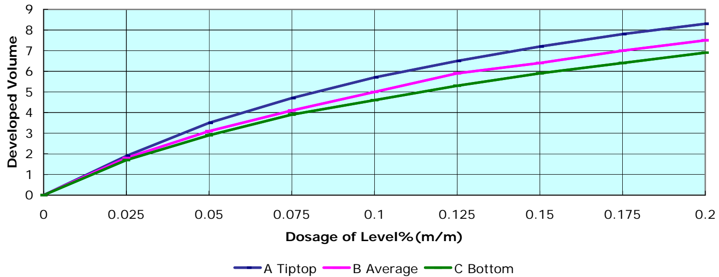
Cetane Increasing Curve of Cetane-707(Diesel Oil)
